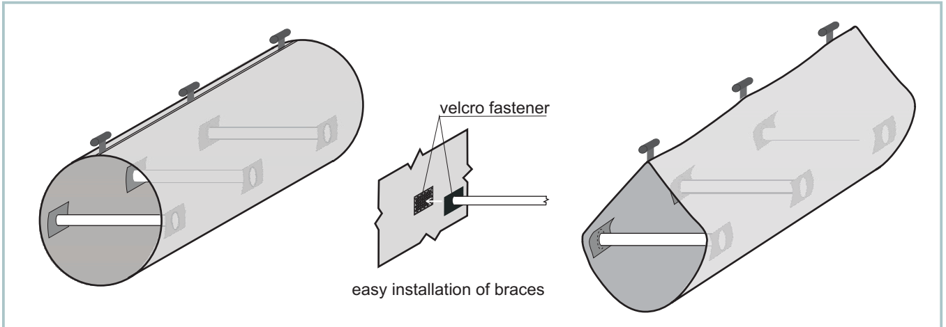
Diffuser with braces - without air supply
